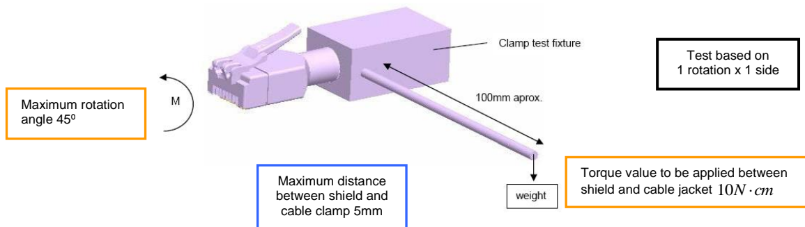
Figure 5: Torsion force test procedure
