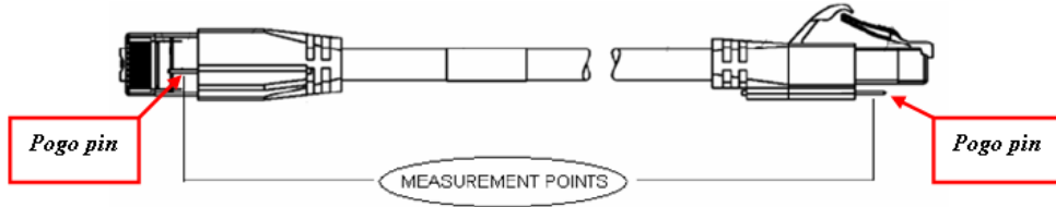
Figure 2: AMPTRAC connection continuity and short-circuit test procedure
