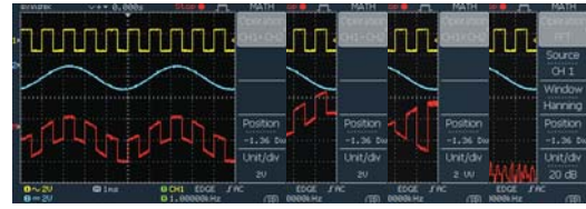
MATH Functions
