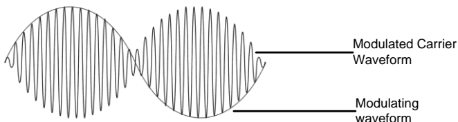
AM (DSB-SC) Waveform
