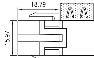
Product assembly drawings
